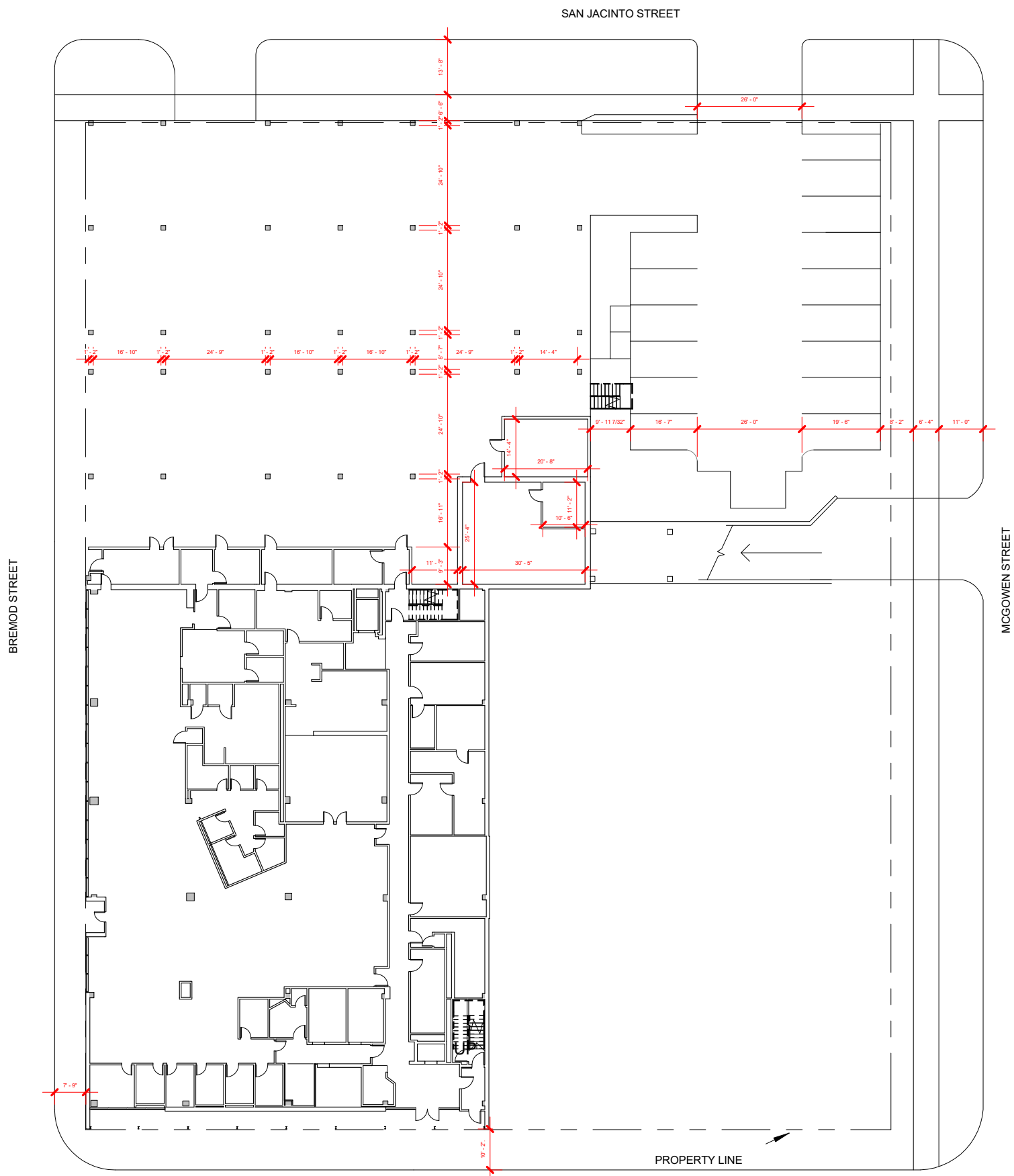
SITE PLAN- FIRST FLOOR PARKING GARAGE
